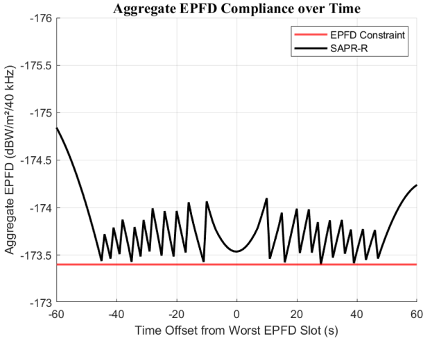
Fig. 7. Aggregate EPFD over time during the critical pass.
