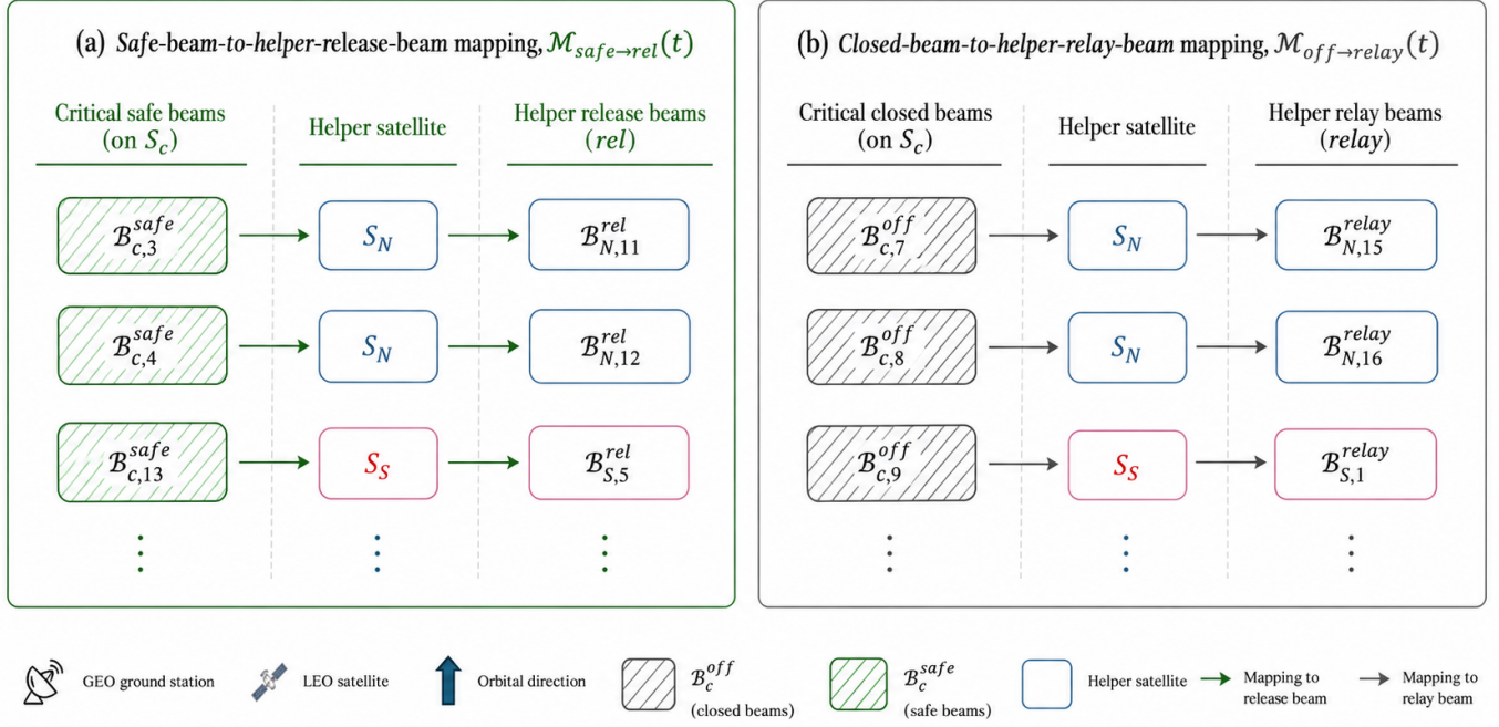
Fig. 4. Beam-pair mapping tables at time slot t . (a) \mathcal{M}_{\text{safe} \rightarrow \text{rel}}(t) : critical safe beams on s^C mapped to helper release beams on s^N/s^S (SAHR). (b) \mathcal{M}_{\text{off} \rightarrow \text{relay}}(t) : critical closed beams mapped to helper relay beams (BPLR).
