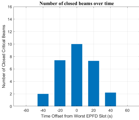
Fig. 8. Number of closed beams over time during the critical pass.
